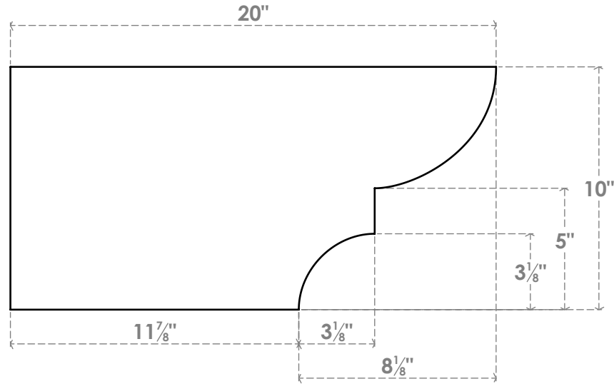
SIDE PROFILE
